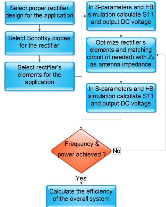
Fig. 2. Design process of the proposed Schottky diode-based dual-band rectifier.
